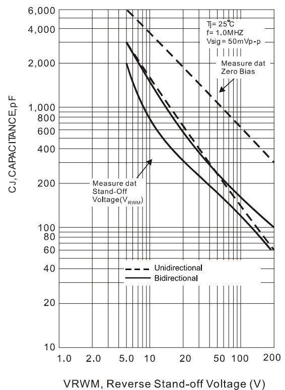
Fig.4 TYPICAL CAPACITANCE
