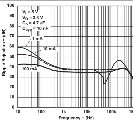
Figure 6-22. Ripple Rejection vs Frequency for Legacy Chip
