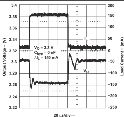
Figure 8-5. Load Transient Response for Legacy Chip
