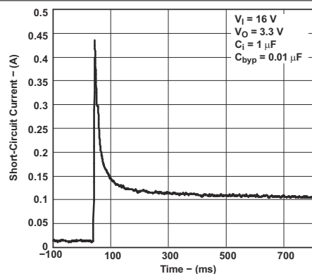
Figure 6-9. Short-Circuit Current vs Time for Legacy Chip
