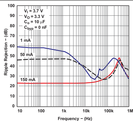
Figure 6-20. Ripple Rejection vs Frequency for Legacy Chip
