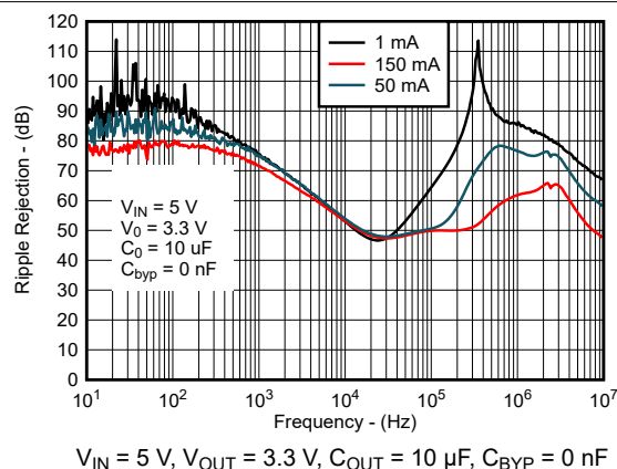
Figure 6-19. Ripple Rejection vs Frequency for New Chip
