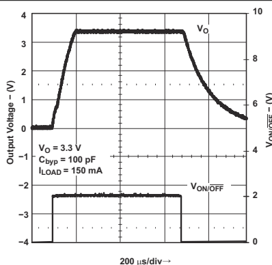
Figure 8-17. Turn-On Time for Legacy Chip
