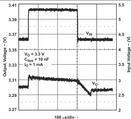
Figure 8-15. Line Transient Response for Legacy Chip
