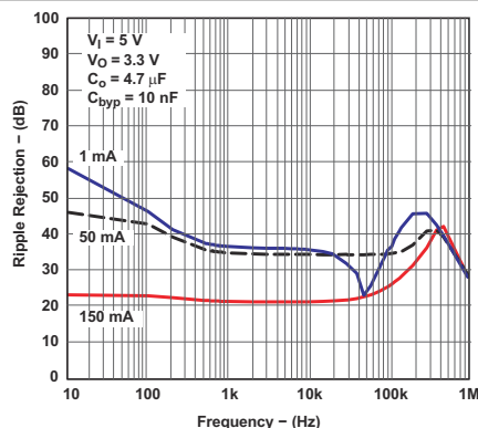
Figure 6-20. Ripple Rejection vs Frequency for Legacy Chip
