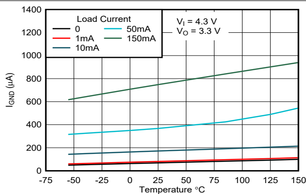
Figure 6-35. Ground-Pin Current vs Temperature for New Chip
