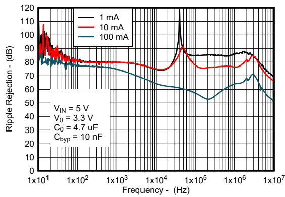
Figure 6-25. Ripple Rejection vs Frequency for New Chip
