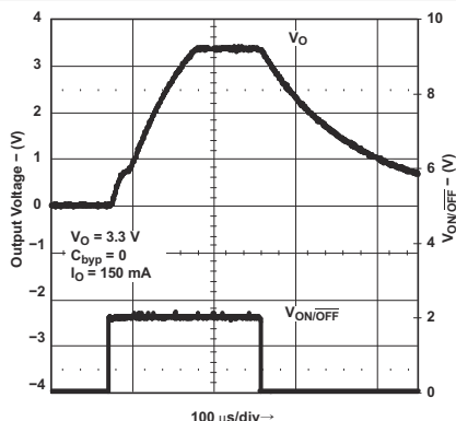
Figure 8-17. Turn-On Time for Legacy Chip
