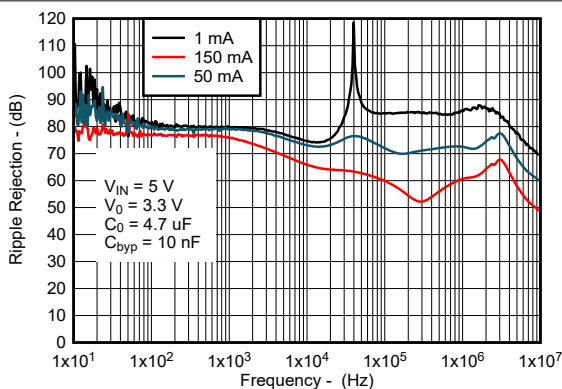
Figure 6-21. Ripple Rejection vs Frequency for New Chip
