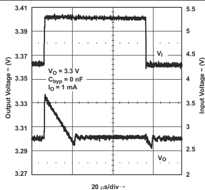
Figure 8-13. Line Transient Response for Legacy Chip
