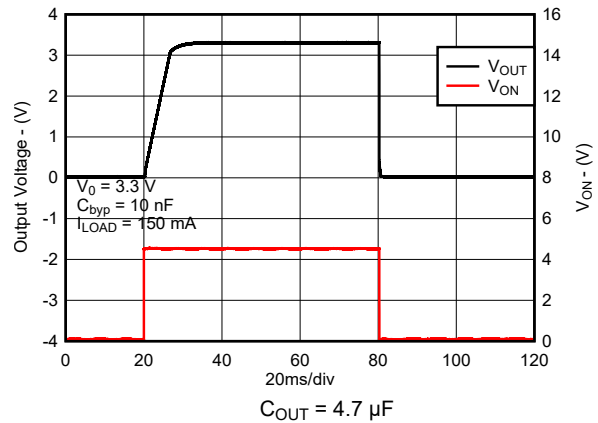
Figure 8-24. Turn-On Time for New Chip
