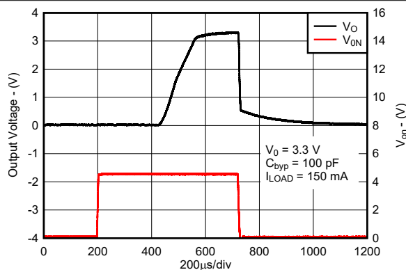
Figure 8-18. Turn-On Time for New Chip
