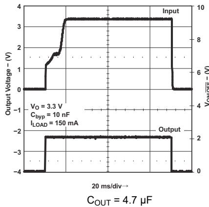
Figure 8-23. Turn-On Time
