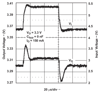
Figure 8-9. Line Transient Response for Legacy Chip
