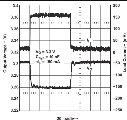
Figure 8-3. Load Transient Response for Legacy Chip
