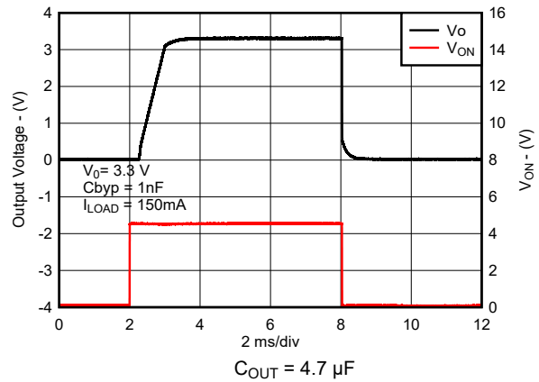
Figure 8-22. Turn-On Time for New Chip
