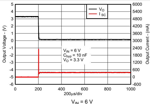
Figure 6-10. Short-Circuit Current vs Time for New Chip
