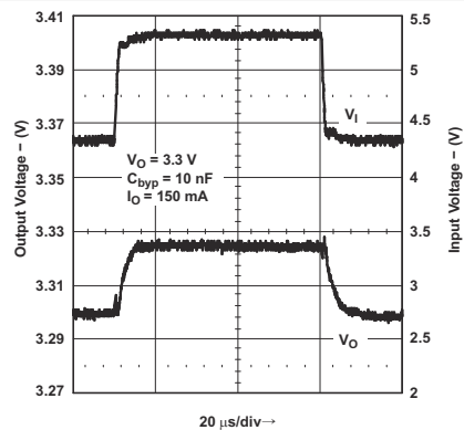
Figure 8-11. Line Transient Response for Legacy Chip
