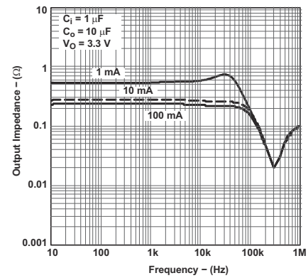
Figure 6-26. Output Impedance vs Frequency for Legacy Chip
