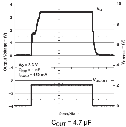
Figure 8-21. Turn-On Time for Legacy Chip
