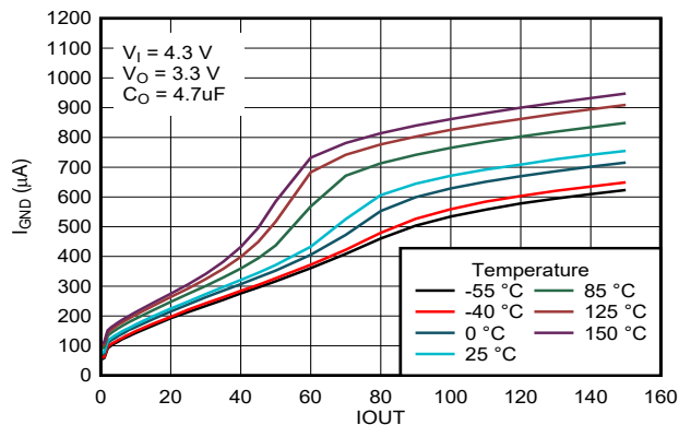
Figure 6-17. Ground Pin Current vs Load Current for New Chip
