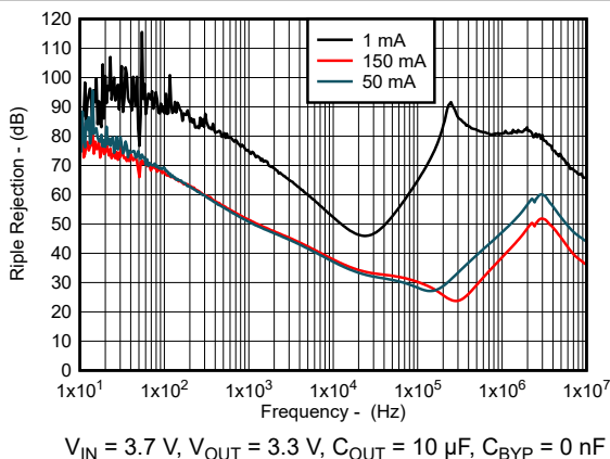
Figure 6-21. Ripple Rejection vs Frequency for New Chip
