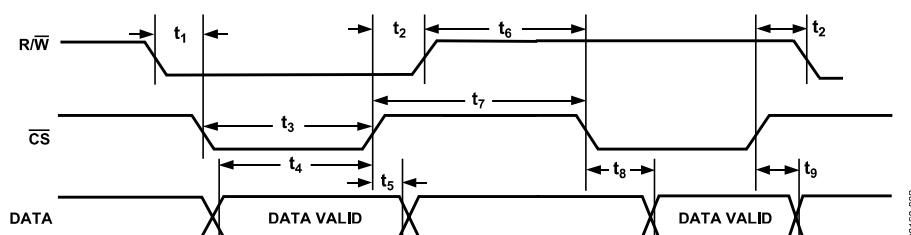
Figure 2. Timing Diagram
