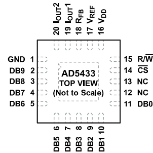
Figure 6. AD5433 Pin Configuration (LFCSP)
