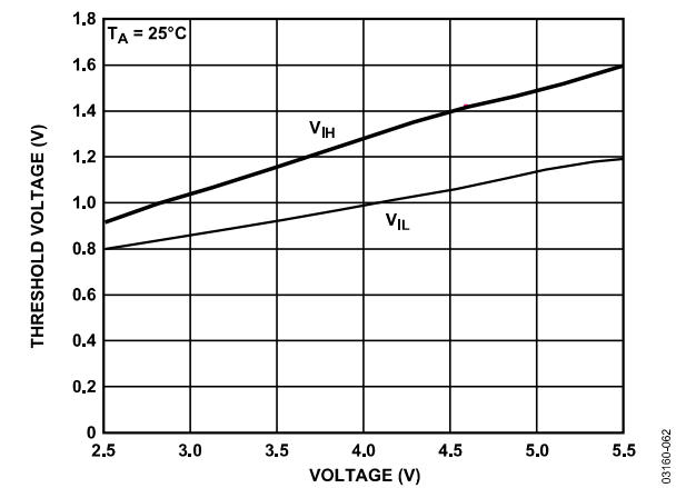
Figure 33. Threshold Voltages vs. Supply Voltage
