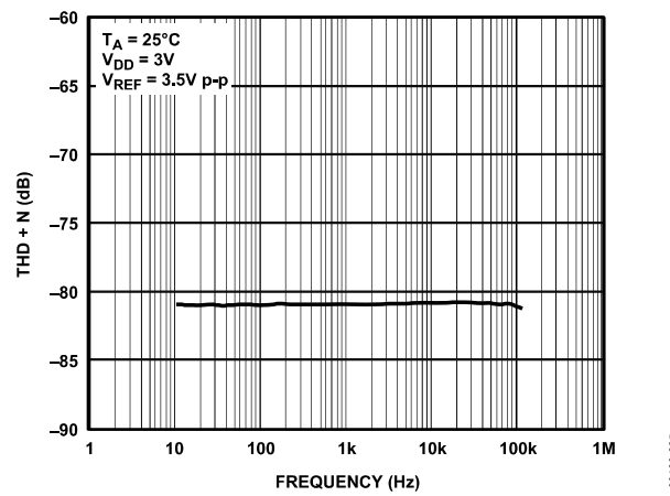
Figure 35. THD and Noise vs. Frequency
