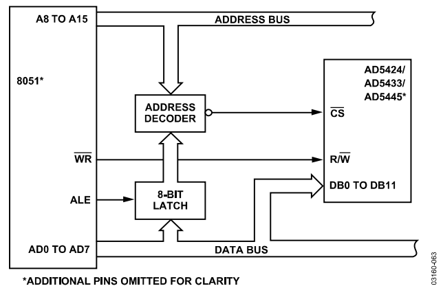
Figure 56. 8xC51-to-AD5424/AD5433/AD5445 Interface
