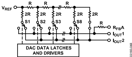
Figure 48. Simplified Ladder
