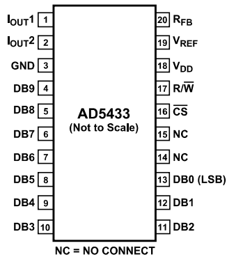
Figure 5. AD5433 Pin Configuration (TSSOP)
