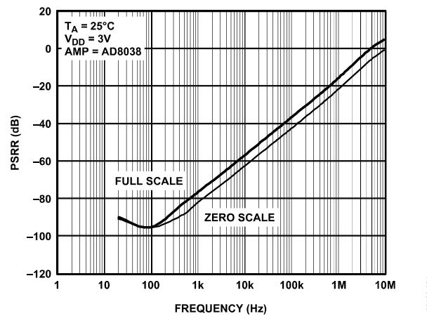
Figure 34. Power Supply Rejection vs. Frequency
