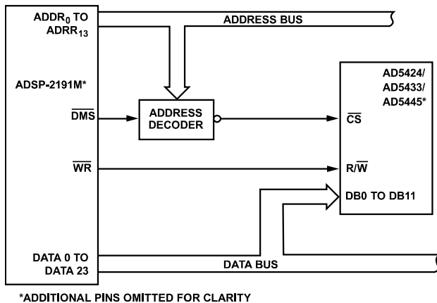
Figure 55. ADSP-2191M-to-AD5424/AD5433/AD5445 Interface
