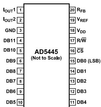
Figure 7. AD5445 Pin Configuration (TSSOP)
