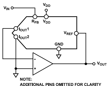
Figure 54. Current-Steering DAC Used as a Divider or Programmable Gain Element
