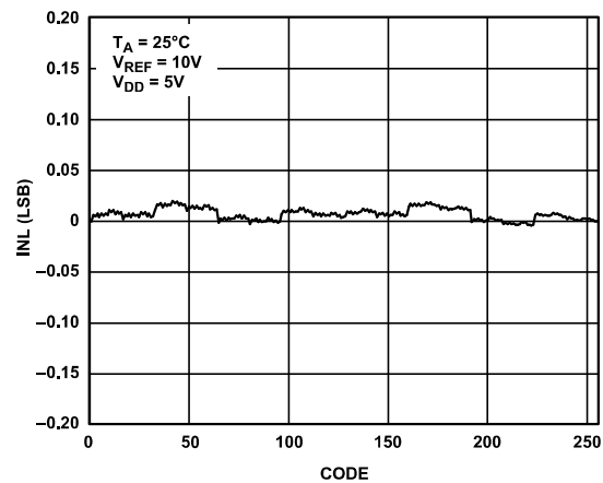
Figure 9. INL vs. Code (8-Bit DAC)
