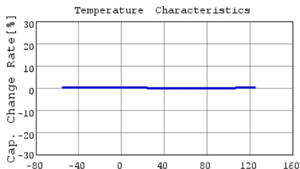
GRM2165C1H273JA01 C-Temp. capchange, DCOV, 1
