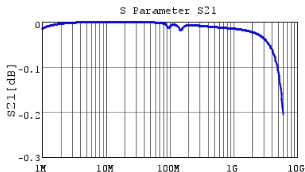
GRM2165C1H273JA01 S21 DCOV, 25degC
