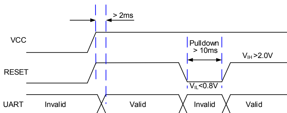
Figure 9: Reset Timing
